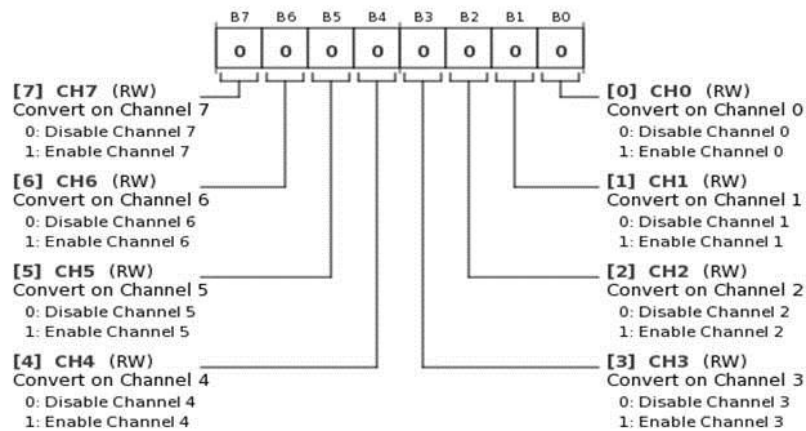
Figure 48. Channel Registers
