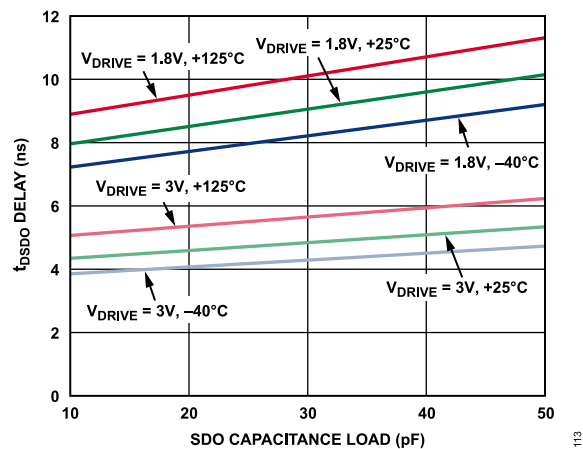
Figure 29. t_{DSO} Delay vs. SDO Capacitance Load and Supply
