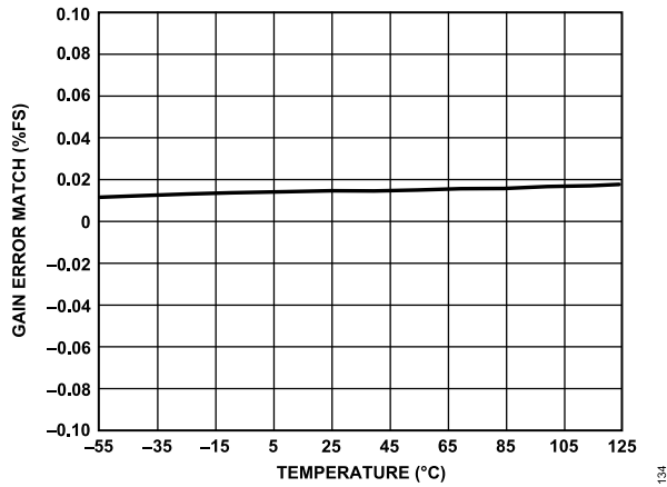
Figure 34. Gain Error Match vs. Temperature
