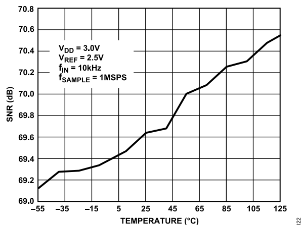
Figure 24. SNR vs. Temperature
