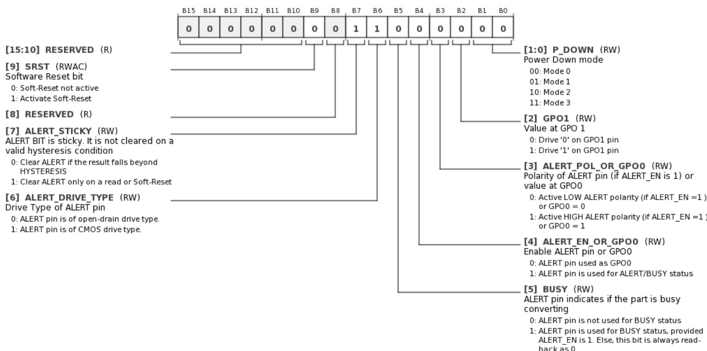
Figure 49. Configuration Register
