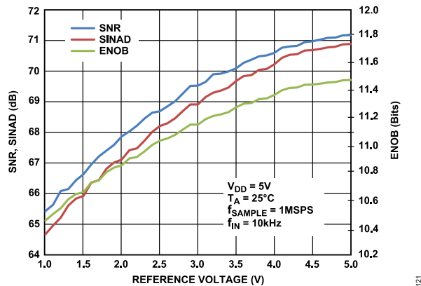
Figure 19. SNR, SINAD, and ENOB vs. Reference Voltage
