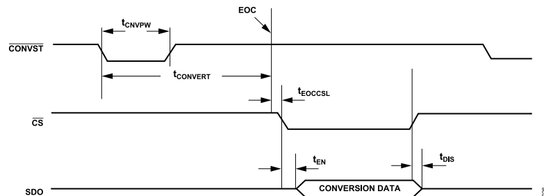
Figure 54. Serial Interface Read Timing in Normal Mode
