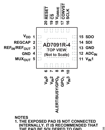
Figure 8. 4-Channel, 20-Lead LFCSP Pin Configuration
