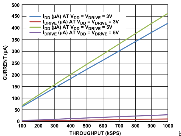
Figure 25. Operating Current vs. Throughput
