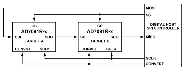
Figure 57. Daisy-Chain Configuration
