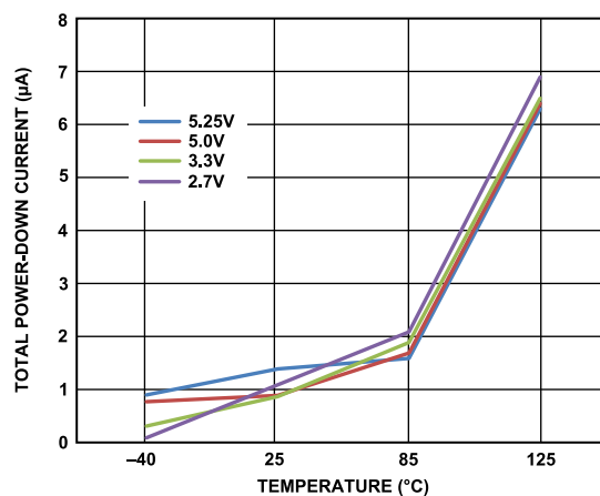
Figure 28. Total Power-Down Current vs. Temperature for Various Supplies
