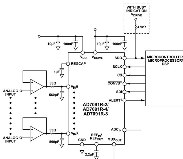
Figure 46. Typical Connection Diagram Without Optional Buffer
