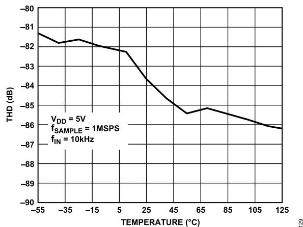
Figure 23. THD vs. Temperature
